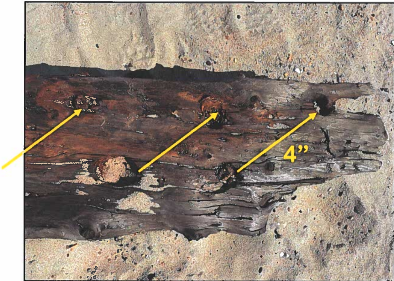
End of timber with treenails. Pattern of fasteners is on a 4" diagonal (Below)
